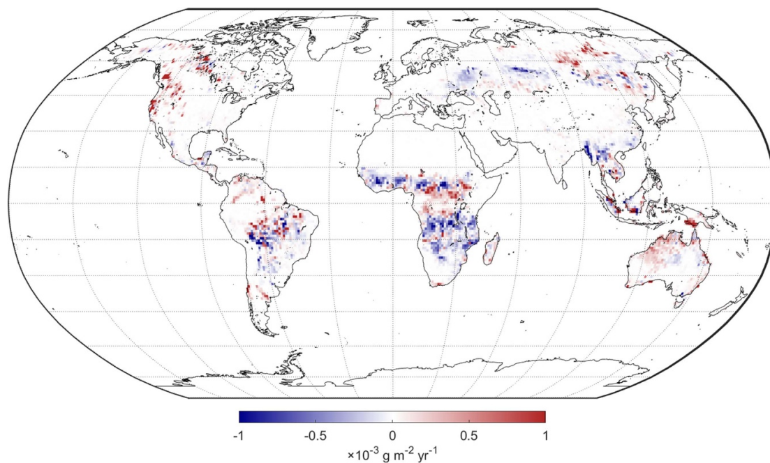
Figure B5. \text{NH}_3 emission trend ( \text{g m}^{-2} \text{ yr}^{-1} ) based on Global Fire Emissions Database (GFED) v4.1s yearly time series during the 2008–2018 period. The trends have been calculated using a standard least squares linear regression fit applied on the yearly data [8].
