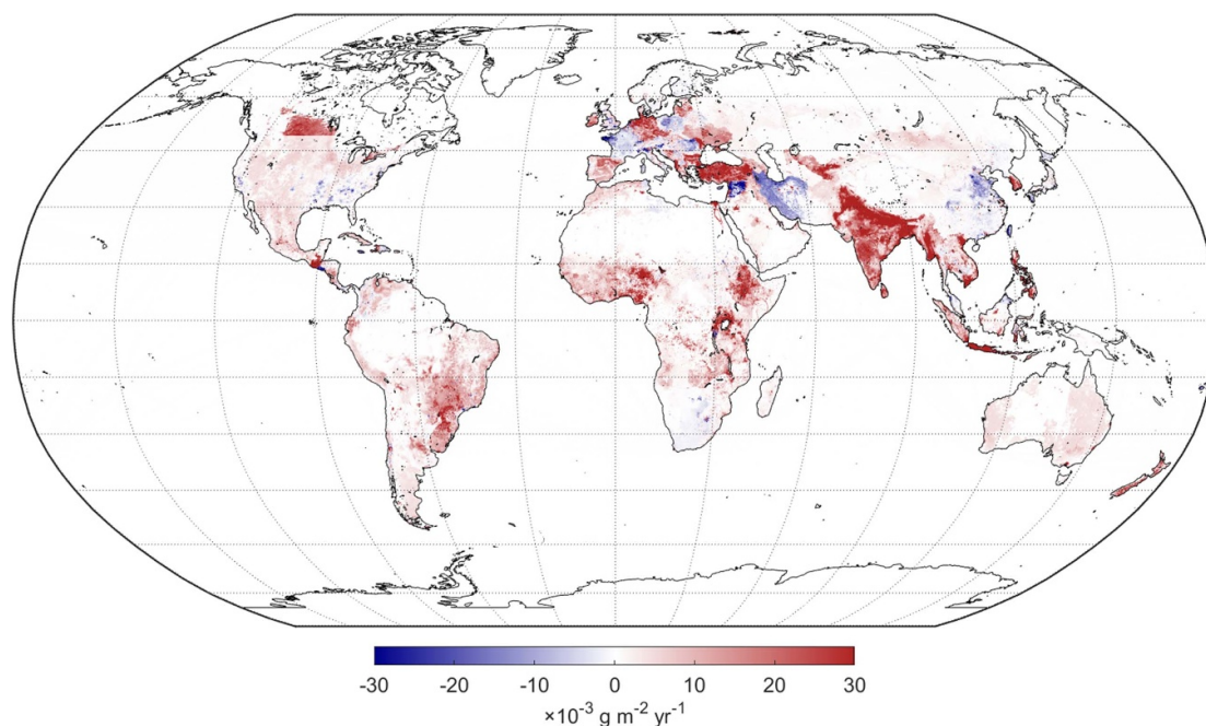
Figure B4. \text{NH}_3 emission trend ( \text{g m}^{-2} \text{ yr}^{-1} ) based on Emission Database for Global Atmospheric Research (EDGAR) v5.0 yearly time series during the 2008–2015 period. The trends have been calculated using a standard least squares linear regression fit applied on the yearly data [6].
